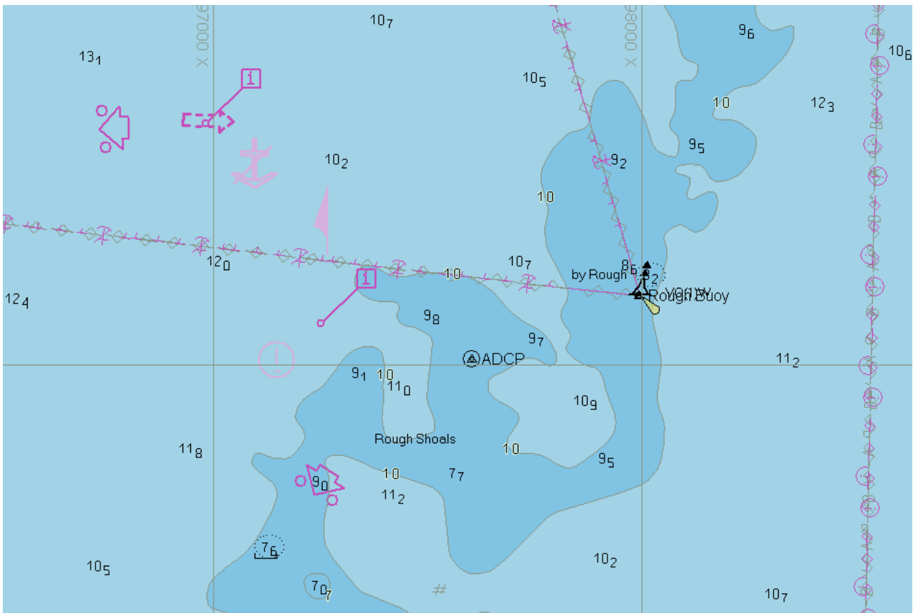
Picture 1: Location of deployed equipment (ADCP) in the vicinity of the Rough Shoals
